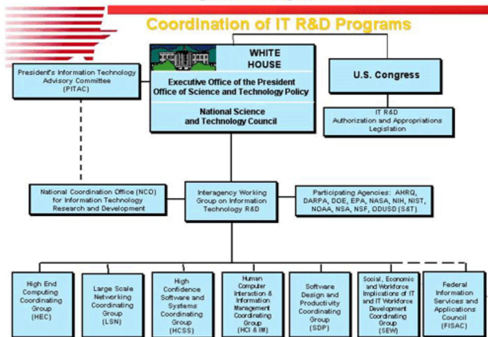
Figure 2 - Program Structure
